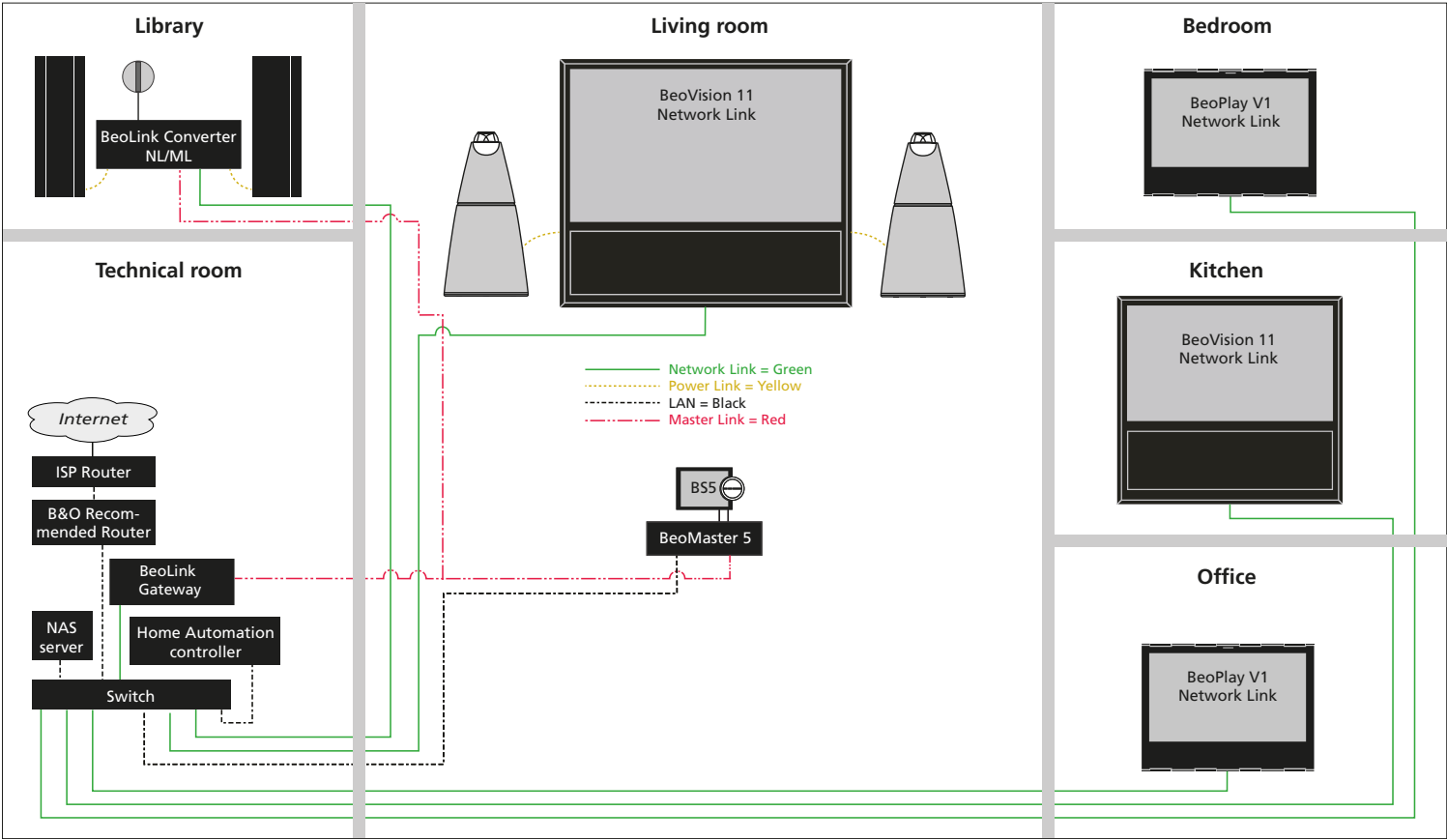
NL scenario 2 - Network Link TV and Master Link audio
